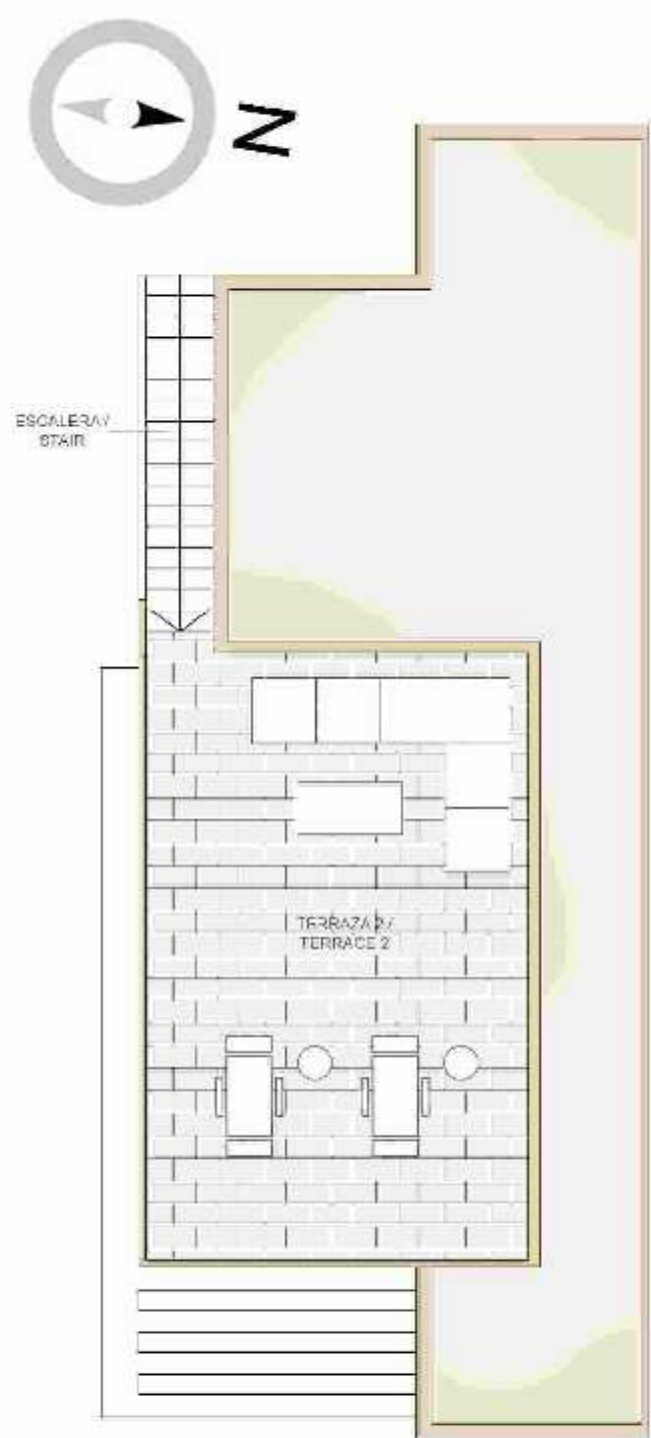
Planta Terraza / Solarium Floor
